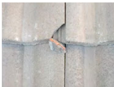
Figure 2. 1/16" bead of adhesive is the ideal amount that will form a proper bond and not squeeze out to block water flow.
